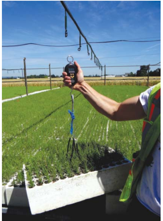
Figure 5. A container fitted with basket hangers has its weight measured with an inexpensive, portable, handheld, digital balance. Photo by R Kasten Dumroese
